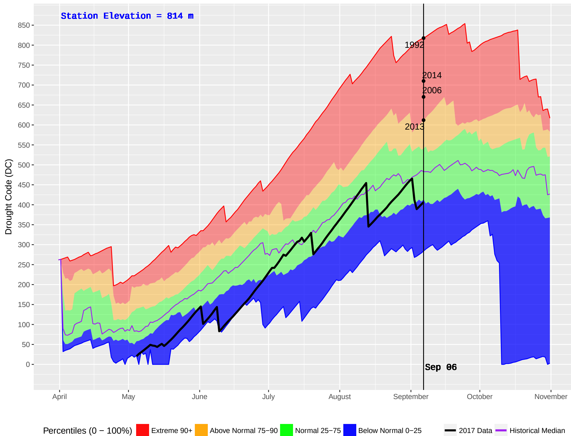
CHILAKO (189) : Historical (1986–2016) and Current (2017) Noon Drought Code (DC)
