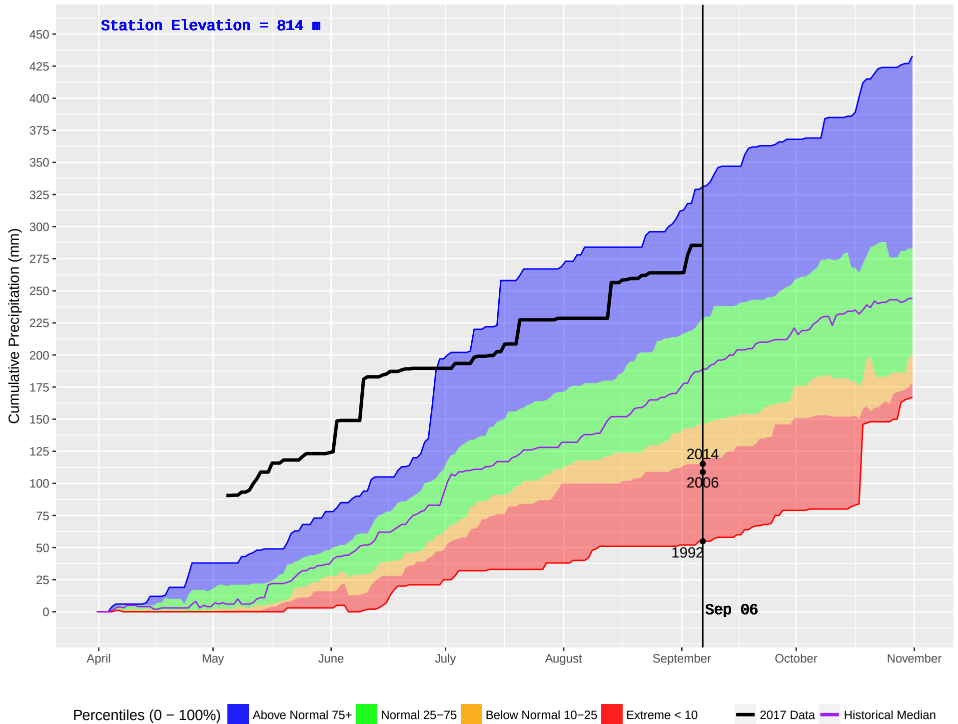
CHILAKO (189) : Historical (1986–2016) and Current (2017) Noon Cumulative Precipitation
