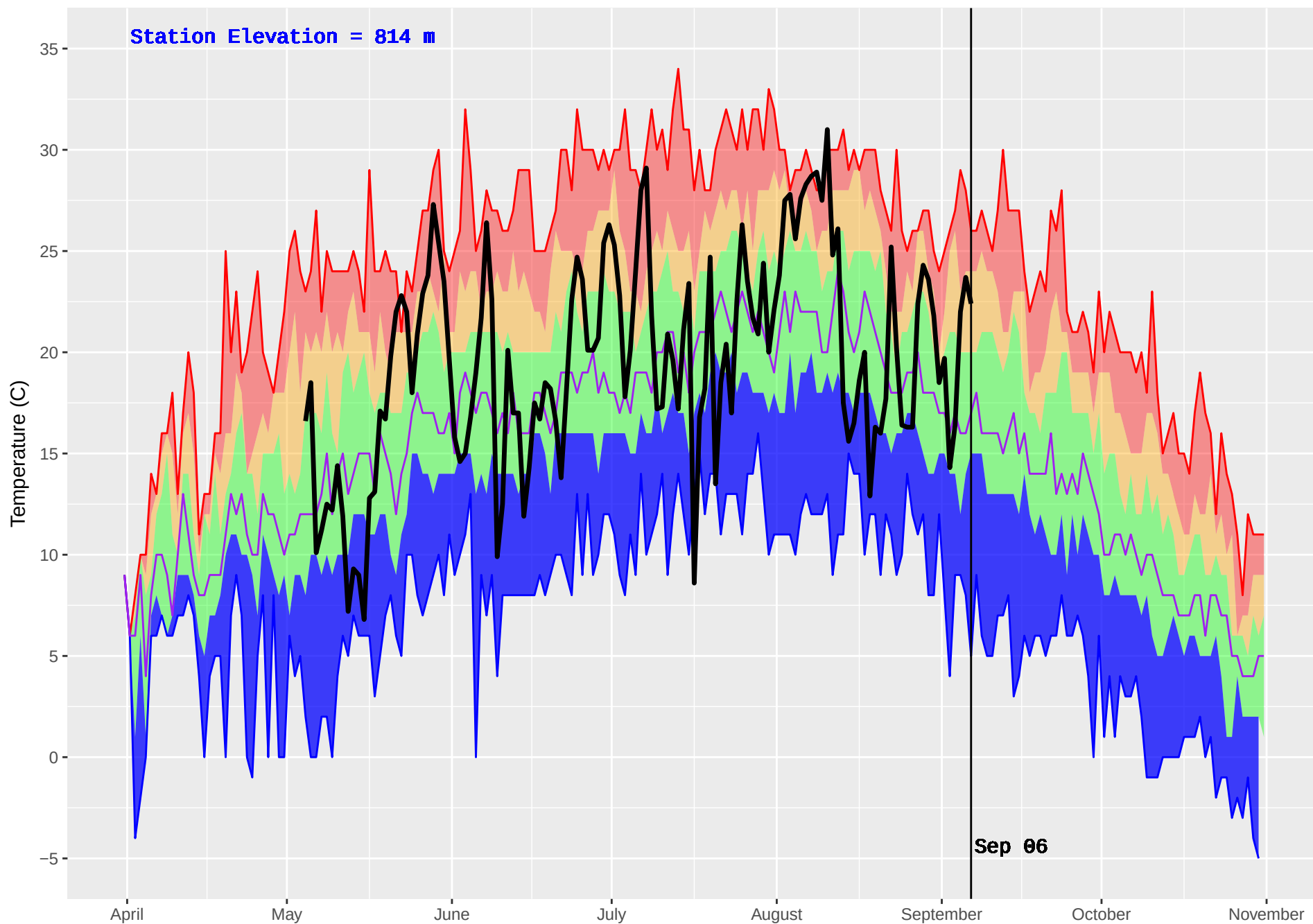
CHILAKO (189) : Historical (1986–2016) and Current (2017) Noon Temperature
